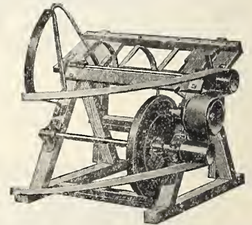
TILTING TABLE POLE SAW Weight, 350 Pounds
